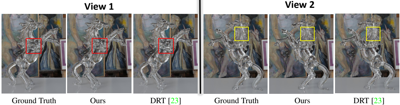
Figure 2: The comparisons of novel view synthesis with \textit{sparsity} = 8 (9 views). After obtaining the reconstruction models via our method and DRT, we render two views of the models via Blender. Compared with DRT, our method produces more accurate renderings (see the red and yellow boxes), which indicates the high quality of our reconstruction.
